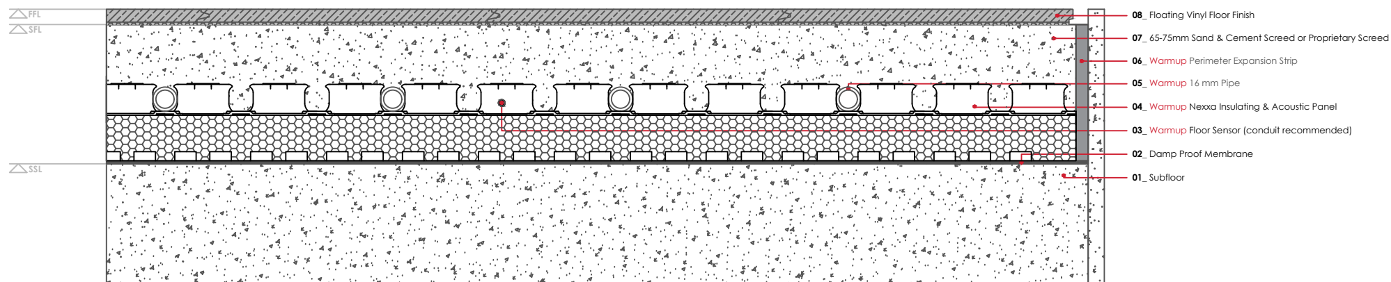
WARMUP NEXXA INSULATING & ACOUSTIC SYSTEM. Vinyl floor finish - floating
