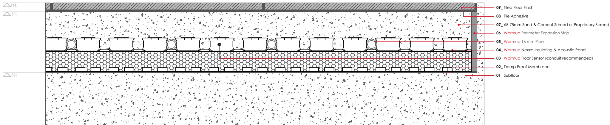
WARMUP NEXXA INSULATING & ACOUSTIC SYSTEM. Tiled floor finish
