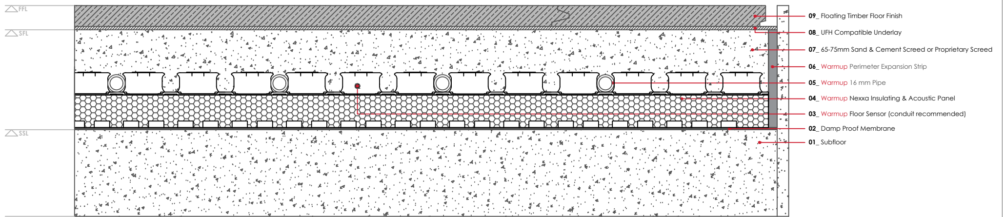
WARMUP NEXXA INSULATING & ACOUSTIC SYSTEM. Floating timber floor finish
