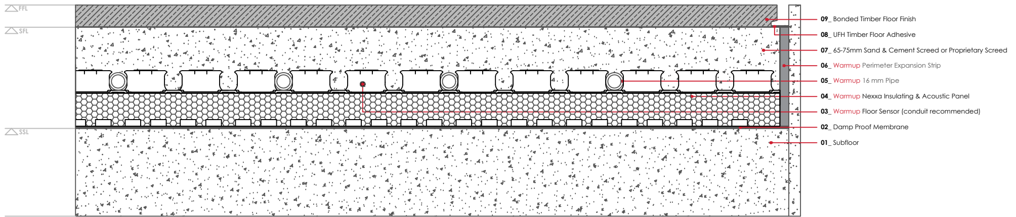
WARMUP NEXXA INSULATING & ACOUSTIC SYSTEM. Bonded timber floor finish
