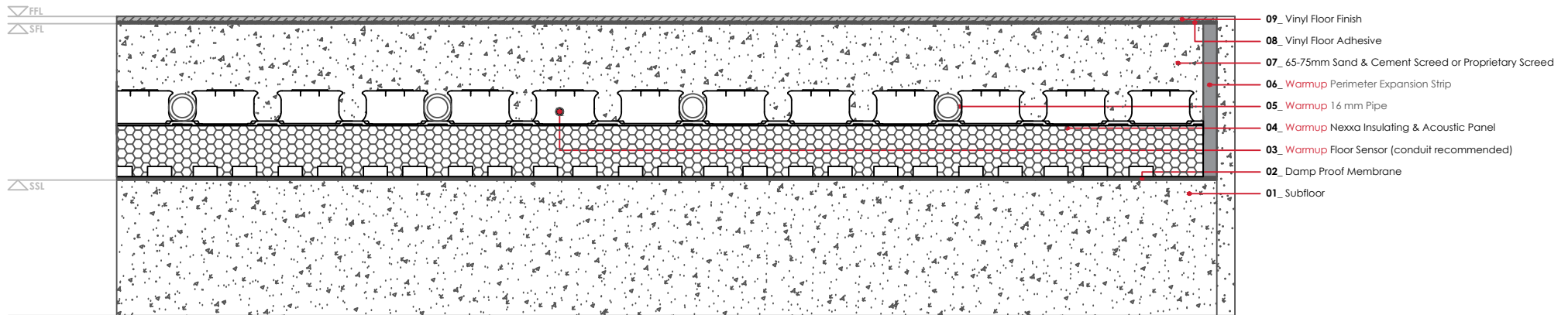
WARMUP NEXXA INSULATING & ACOUSTIC SYSTEM. Vinyl floor finish - glued
