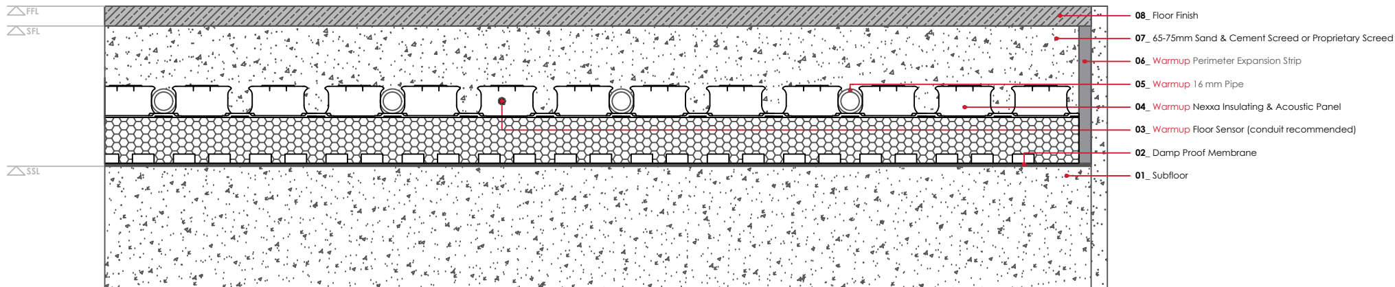
WARMUP NEXXA INSULATING & ACOUSTIC SYSTEM. Standard Detail
