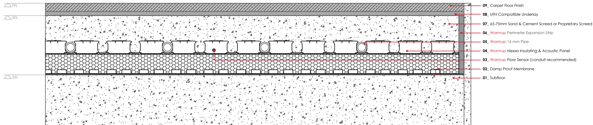
WARMUP NEXXA INSULATING & ACOUSTIC SYSTEM. Carpet floor finish
