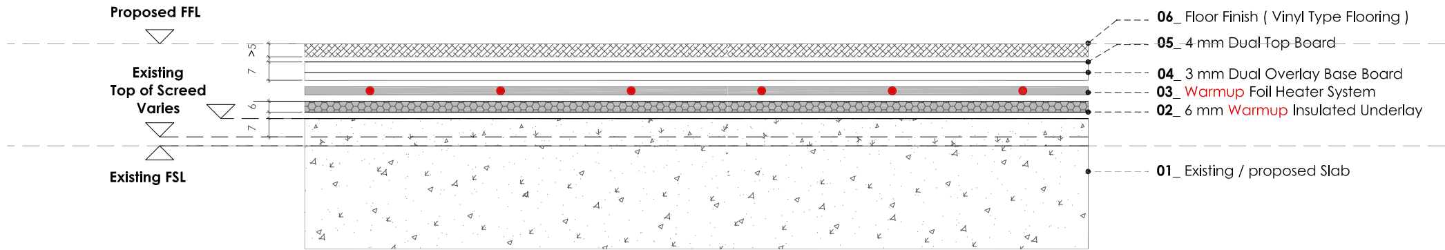
WARMUP UNDERFLOOR HEATING FOIL HEATER SYSTEM ( VINYL TYPE FLOORING)
