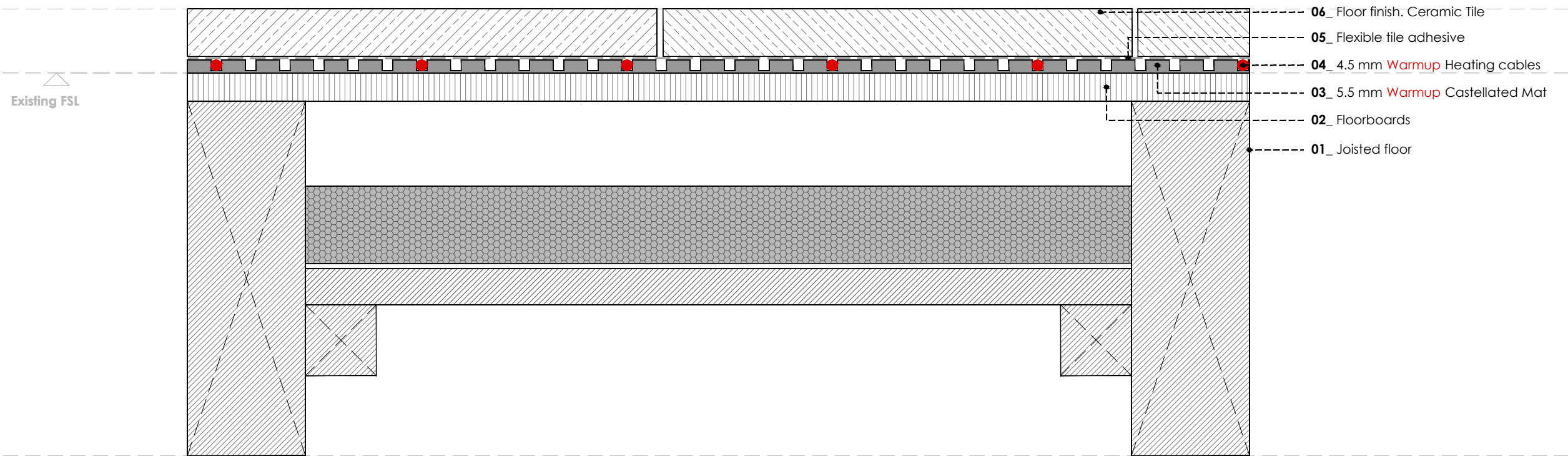
WARMUP CASTELLATED MAT SYSTEM. TIMBER SUBFLOOR AND TILES
